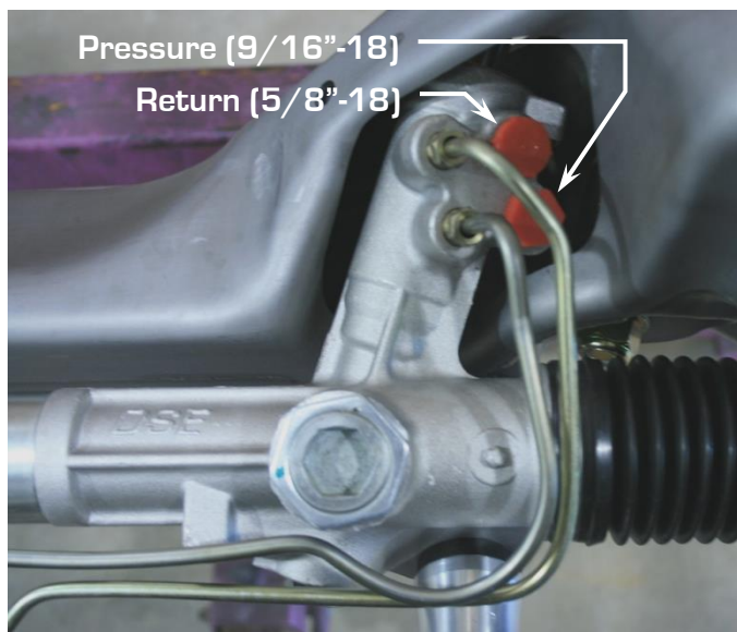
Figure 1 – Pressure and Return Port Locations
