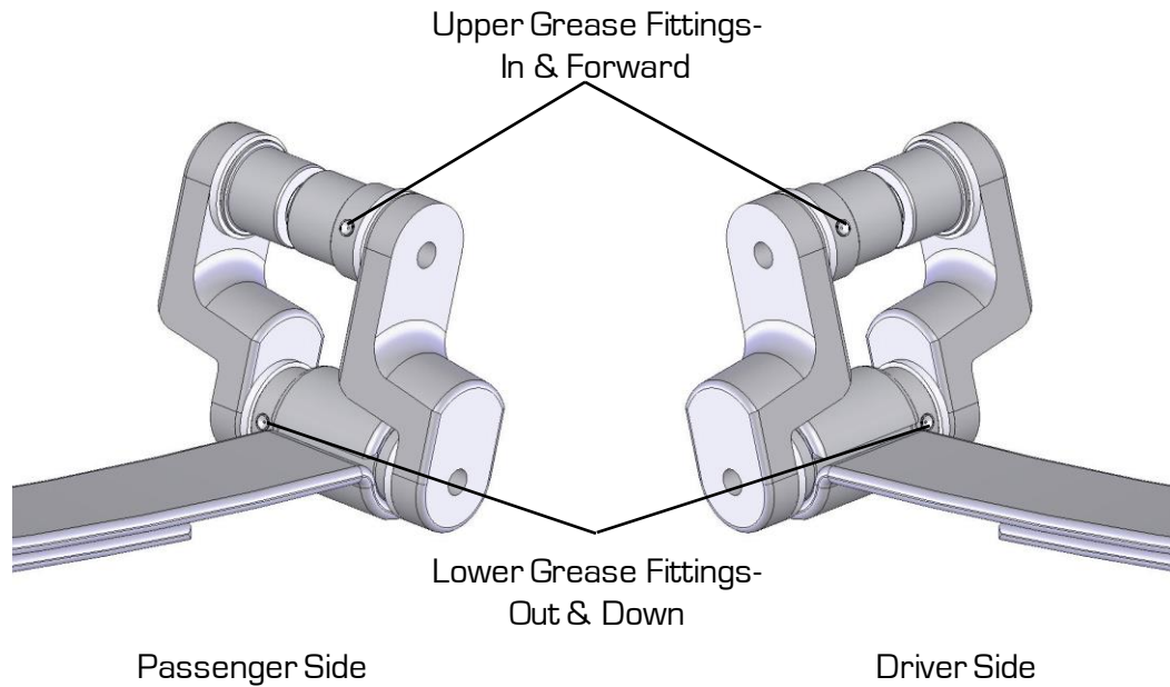
Figure 2. Delrin Bushing Positioning (Normal or Offset Shackles)
