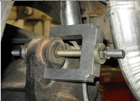
Figure 1 - Removal of the Axle Bushing
